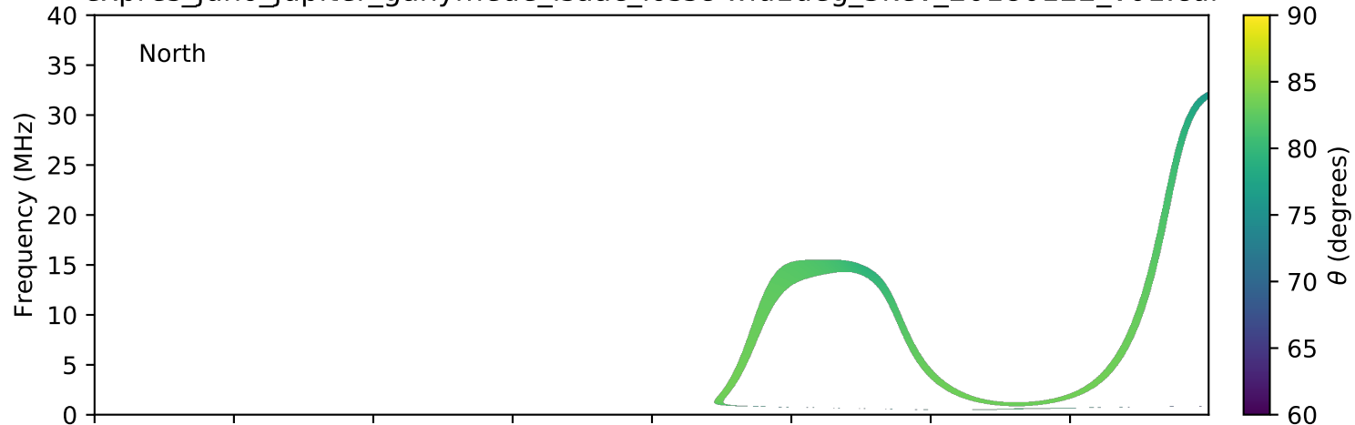
expres_juno_jupiter_ganymede_isaac_lossc-wid1deg_3kev_20180122_v01.cdf
