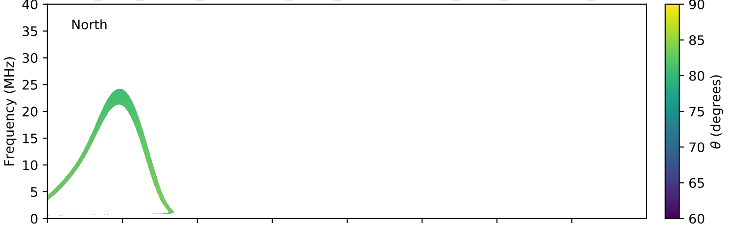
expres_juno_jupiter_ganymede_isaac_lossc-wid1deg_3kev_20180118_v01.cdf
