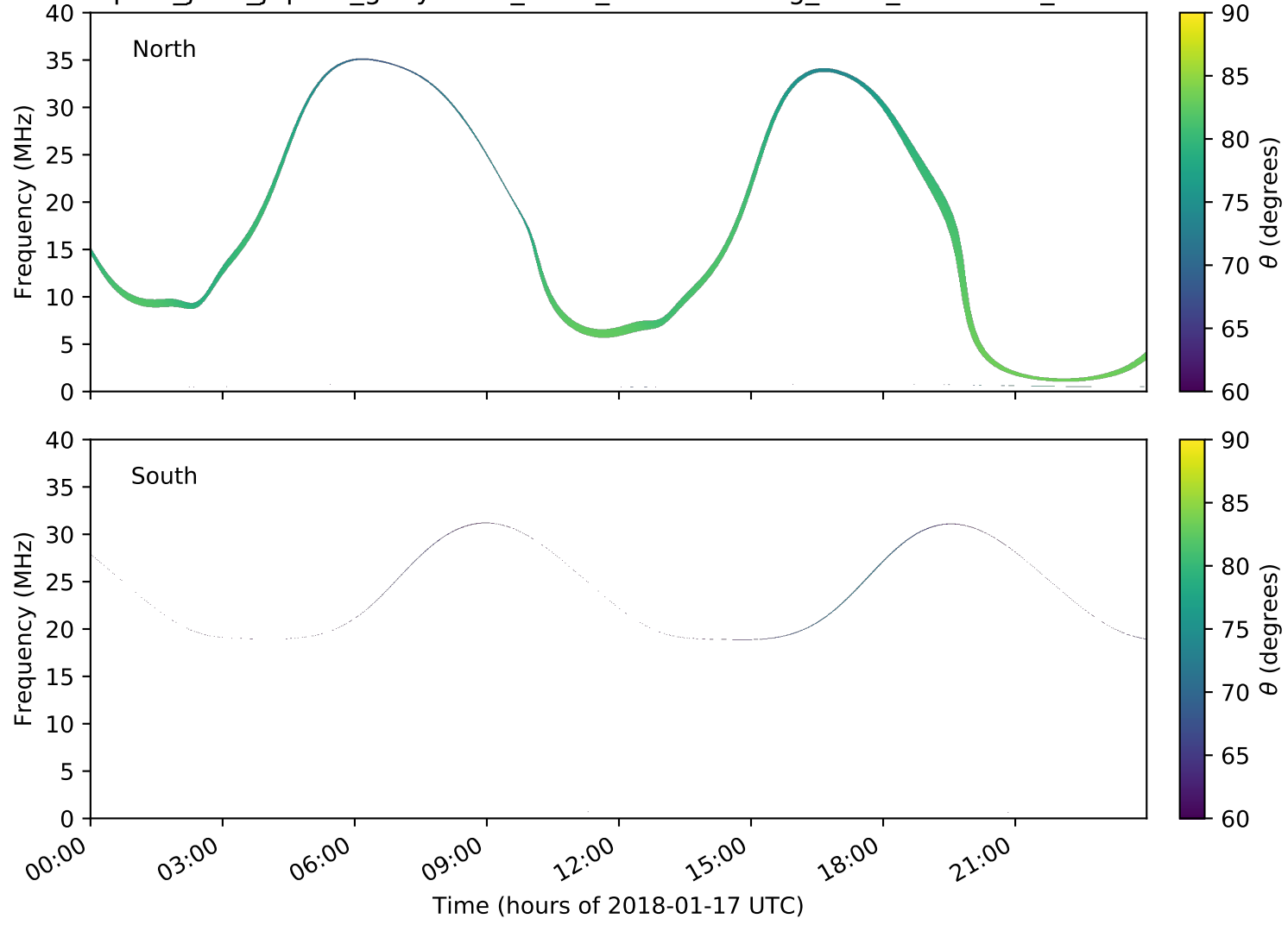
expres_juno_jupiter_ganymede_isaac_lossc-wid1deg_3kev_20180117_v01.cdf
