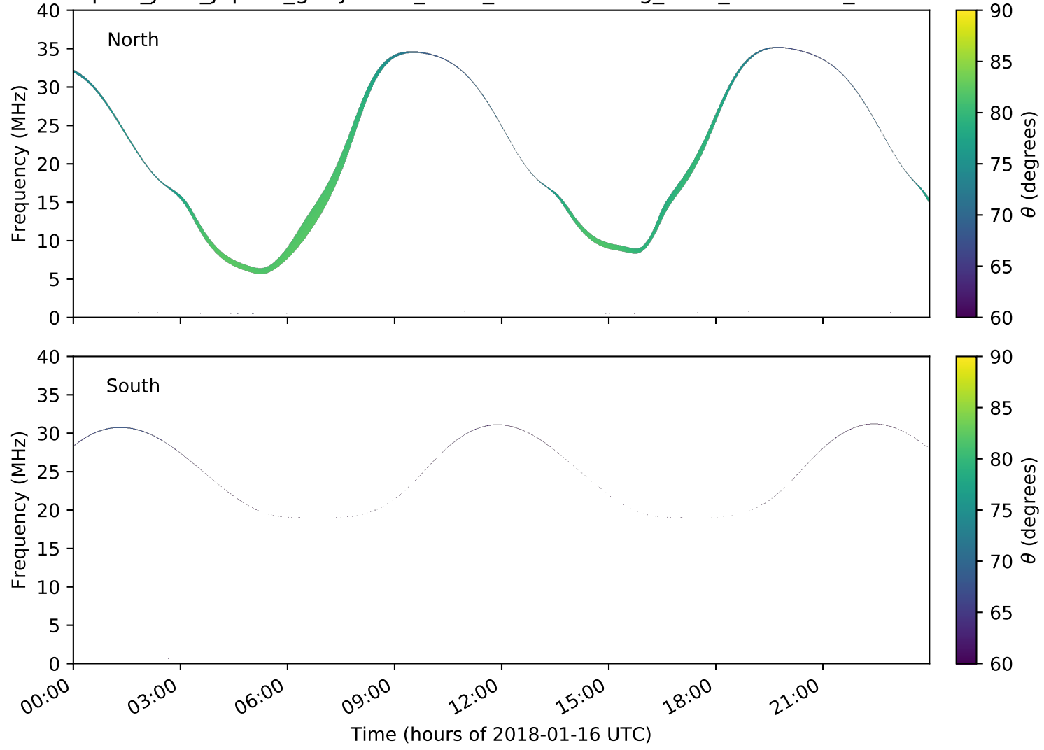
expres_juno_jupiter_ganymede_isaac_lossc-wid1deg_3kev_20180116_v01.cdf
