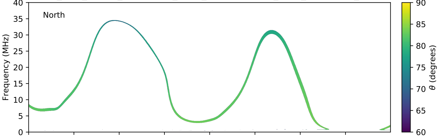
expres_juno_jupiter_ganymede_isaac_lossc-wid1deg_3kev_20180110_v01.cdf
