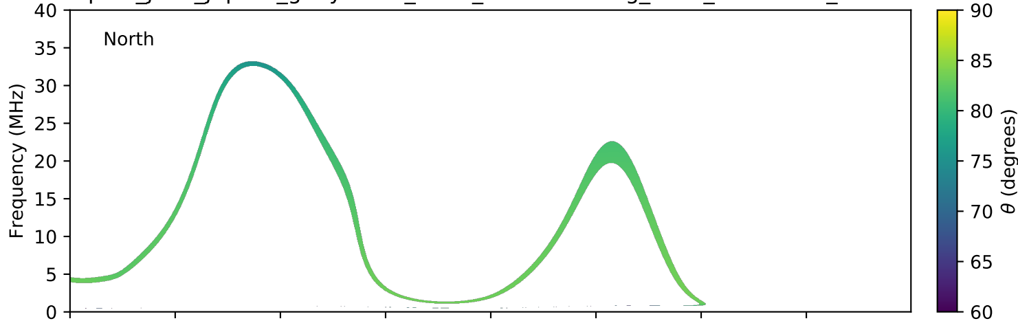
expres_juno_jupiter_ganymede_isaac_lossc-wid1deg_3kev_20180103_v01.cdf
