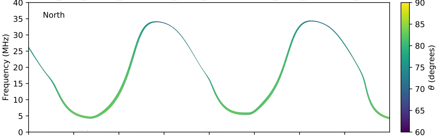
expres_juno_jupiter_ganymede_isaac_lossc-wid1deg_3kev_20180102_v01.cdf
