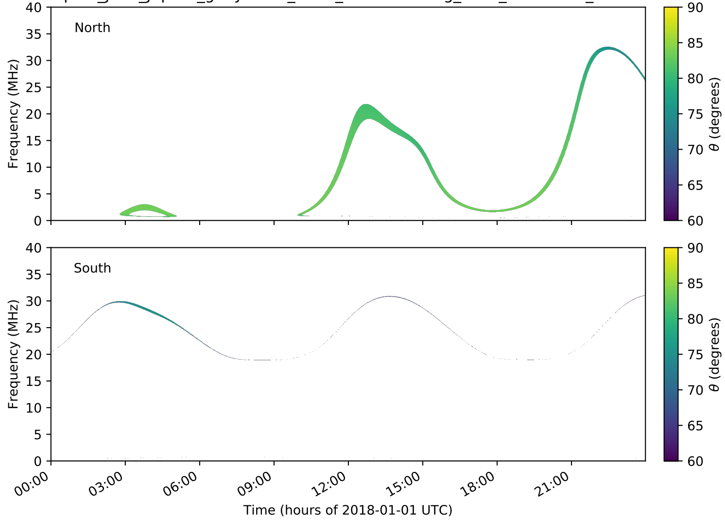
expres_juno_jupiter_ganymede_isaac_lossc-wid1deg_3kev_20180101_v01.cdf
