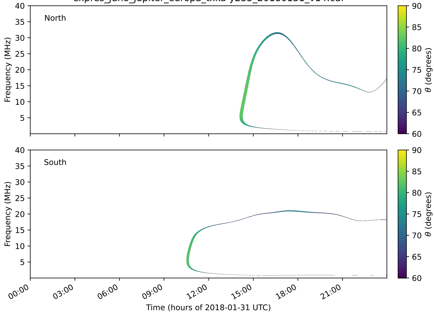
expres_juno_jupiter_europa_txka-y235_20180131_v14.cdf
