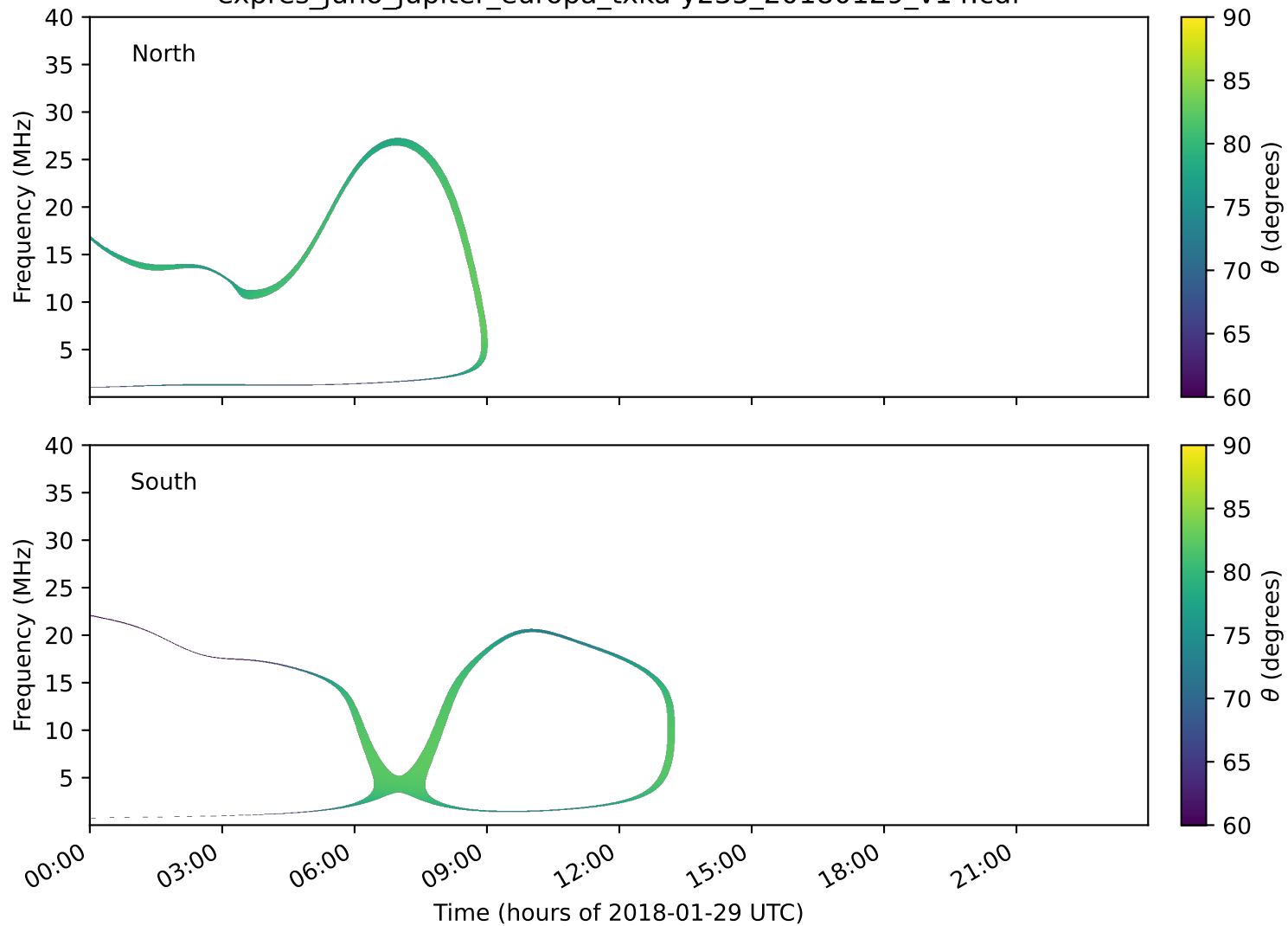
expres_juno_jupiter_europa_txka-y235_20180129_v14.cdf
