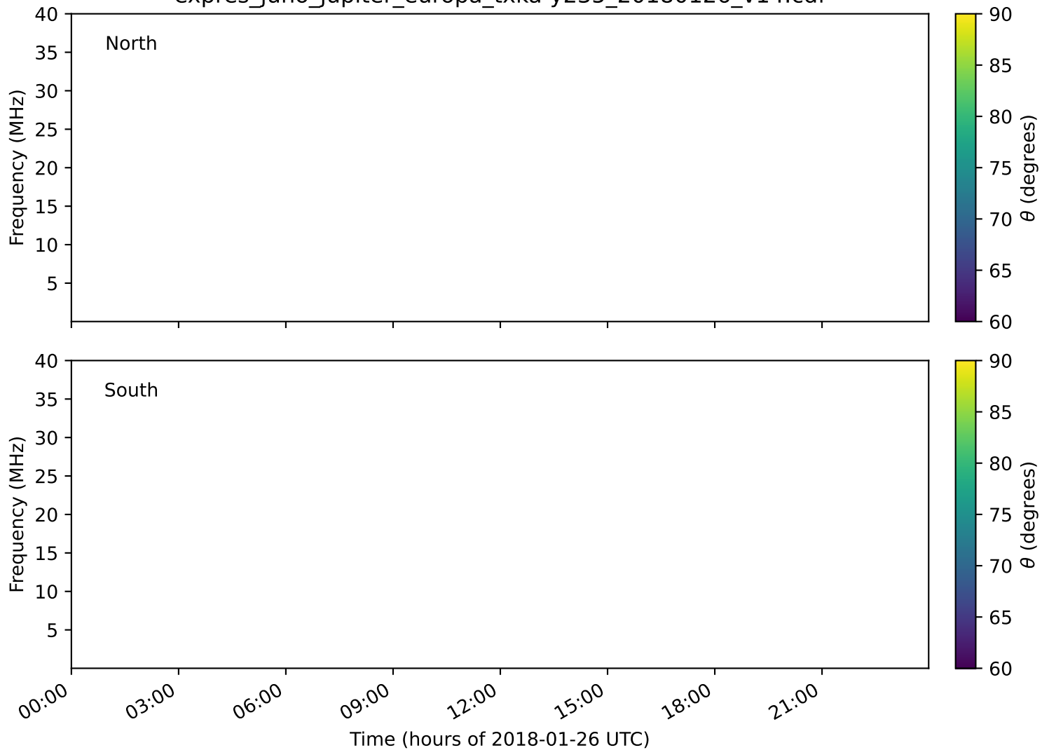
expres_juno_jupiter_europa_txka-y235_20180126_v14.cdf
