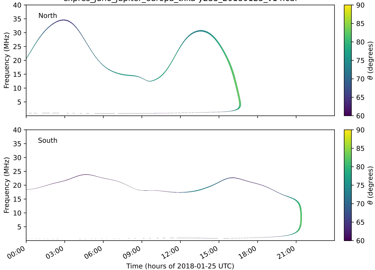
expres_juno_jupiter_europa_txka-y235_20180125_v14.cdf
