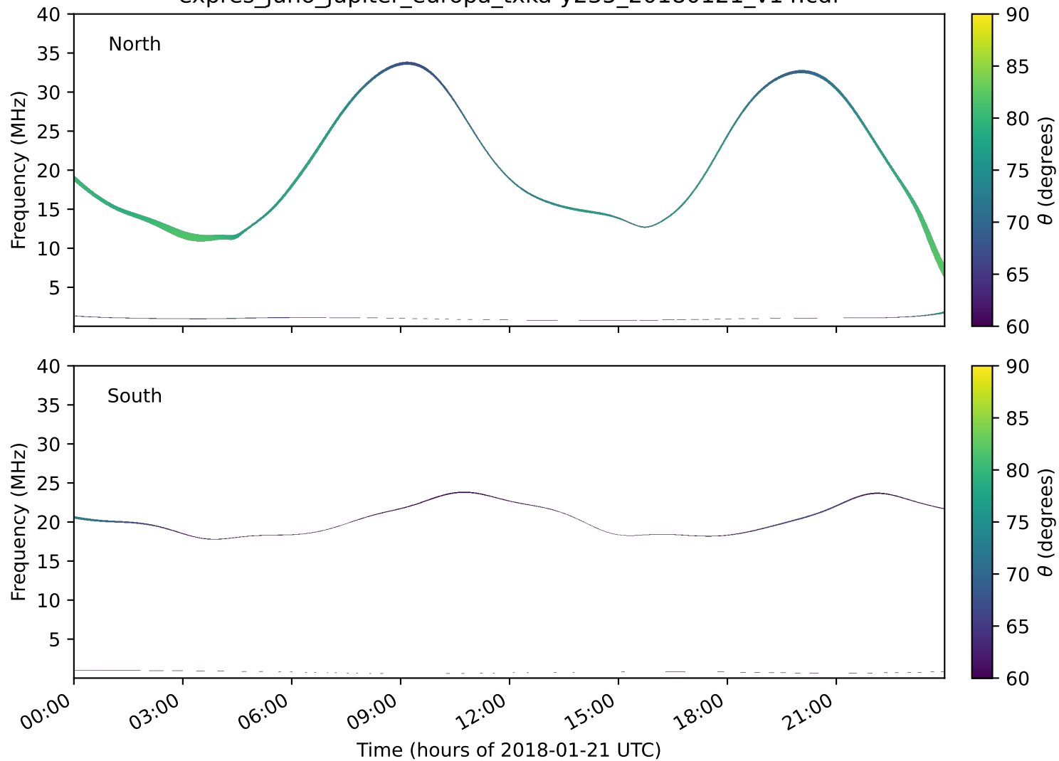
expres_juno_jupiter_europa_txka-y235_20180121_v14.cdf
