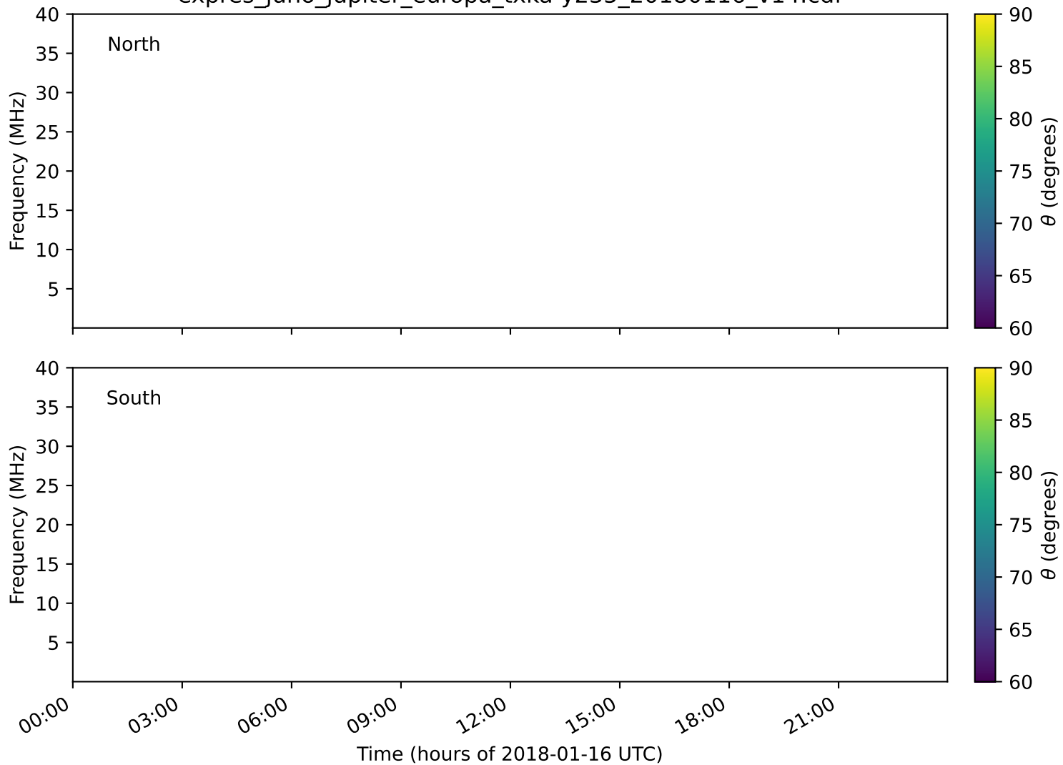
expres_juno_jupiter_europa_txka-y235_20180116_v14.cdf
