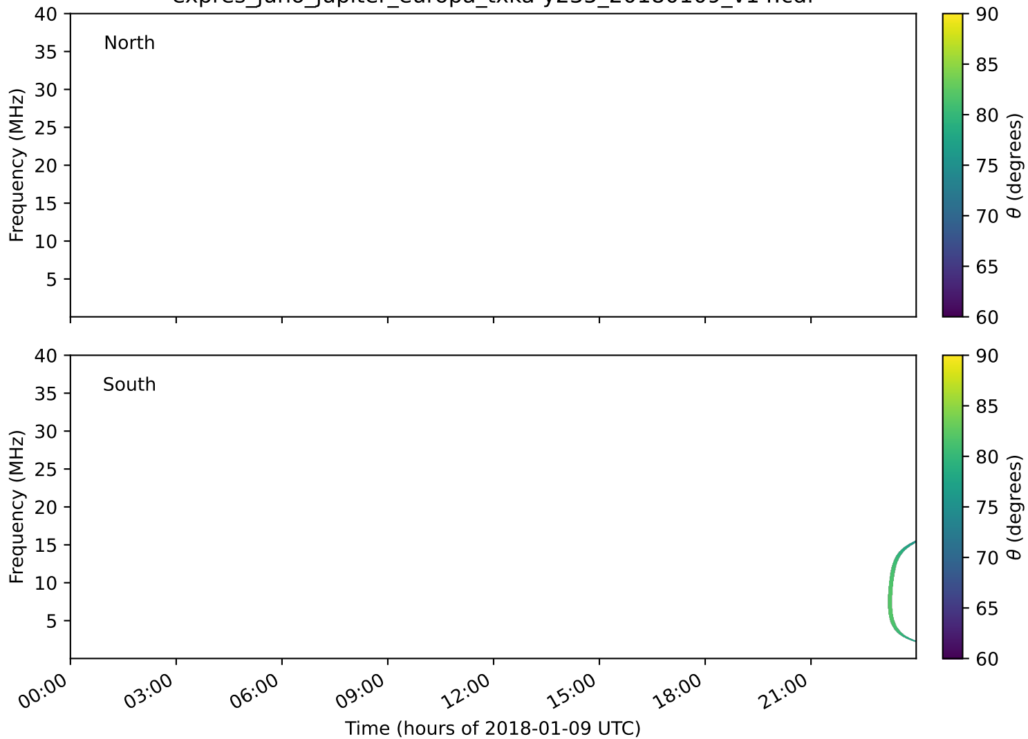
expres_juno_jupiter_europa_txka-y235_20180109_v14.cdf
