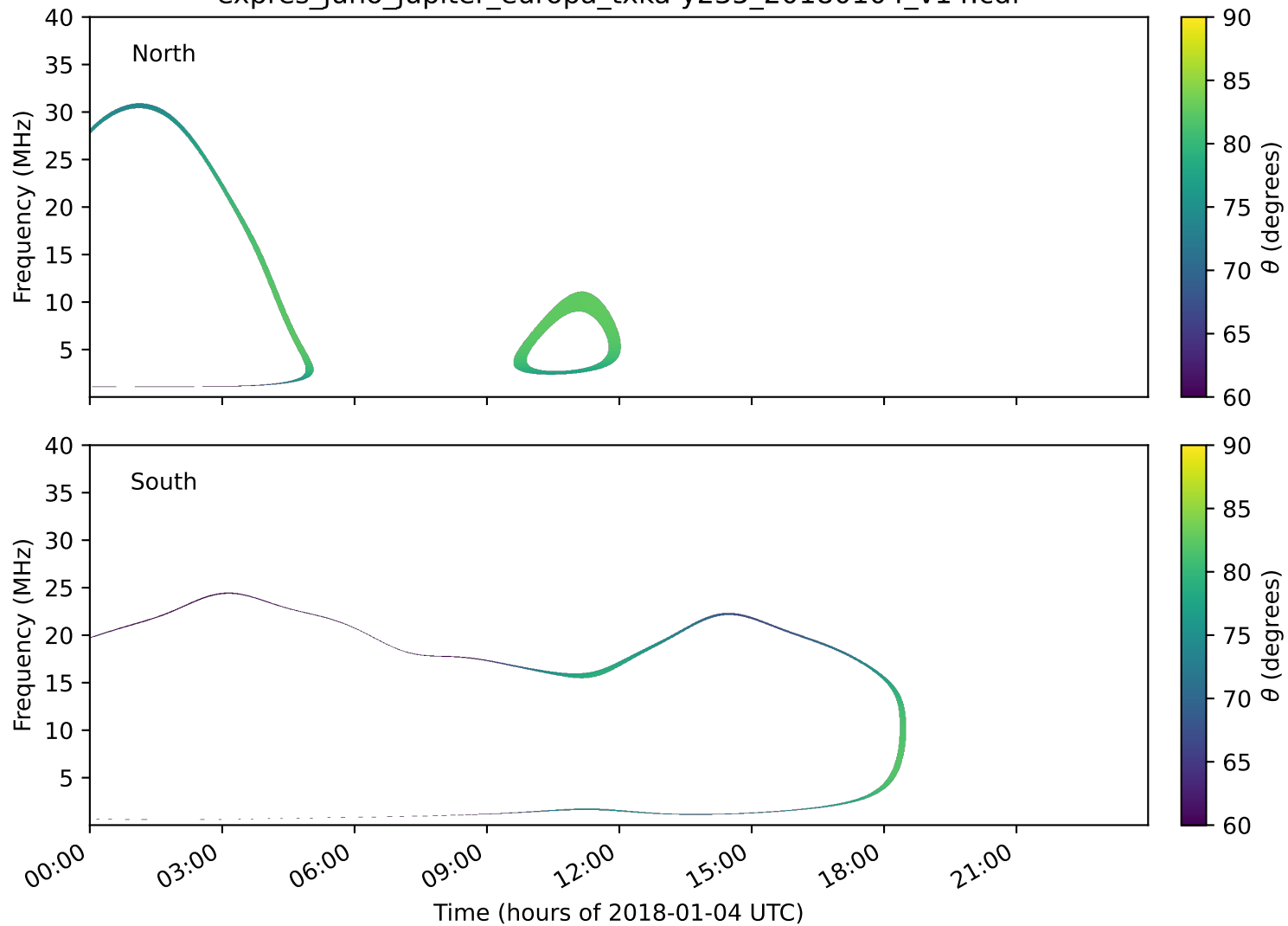
expres_juno_jupiter_europa_txka-y235_20180104_v14.cdf
