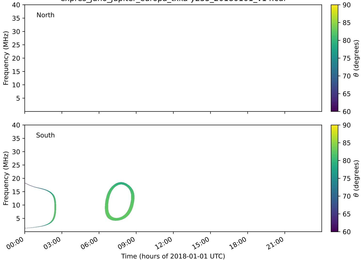
expres_juno_jupiter_europa_txka-y235_20180101_v14.cdf
