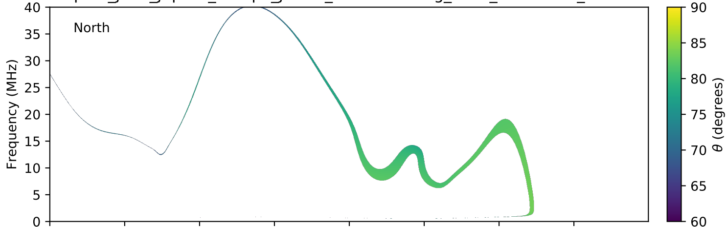
expres_juno_jupiter_europa_jrm09_lossc-wid1deg_3kev_20180131_v01.cdf
