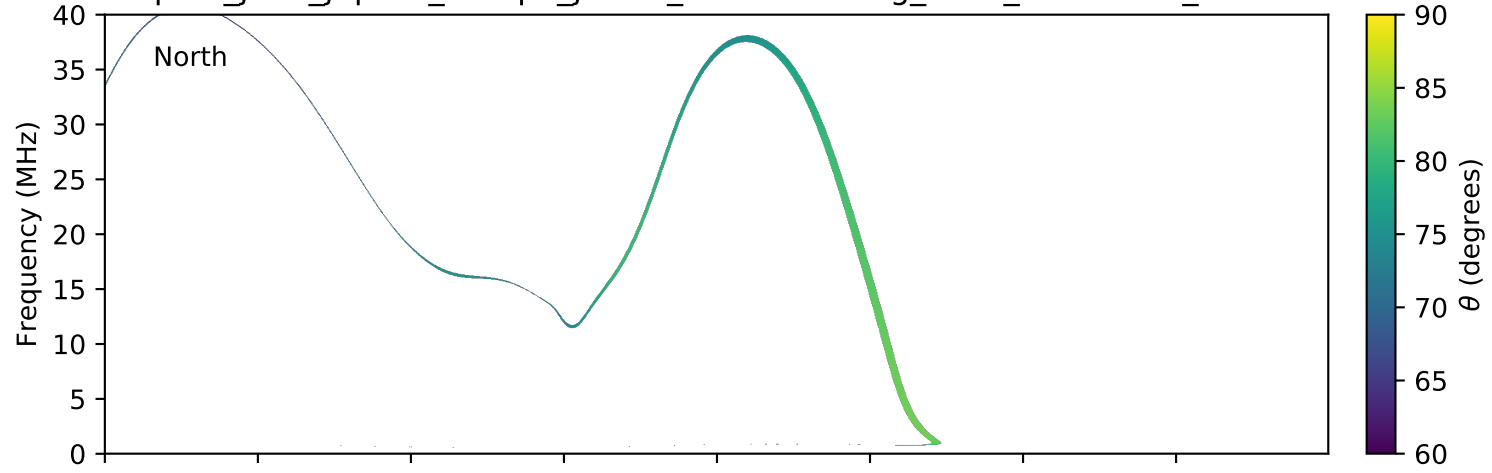
expres_juno_jupiter_europa_jrm09_lossc-wid1deg_3kev_20180130_v01.cdf
