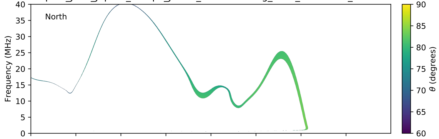
expres_juno_jupiter_europa_jrm09_lossc-wid1deg_3kev_20180129_v01.cdf
