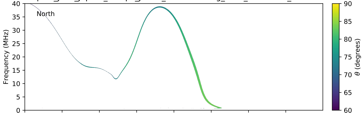
expres_juno_jupiter_europa_jrm09_lossc-wid1deg_3kev_20180128_v01.cdf
