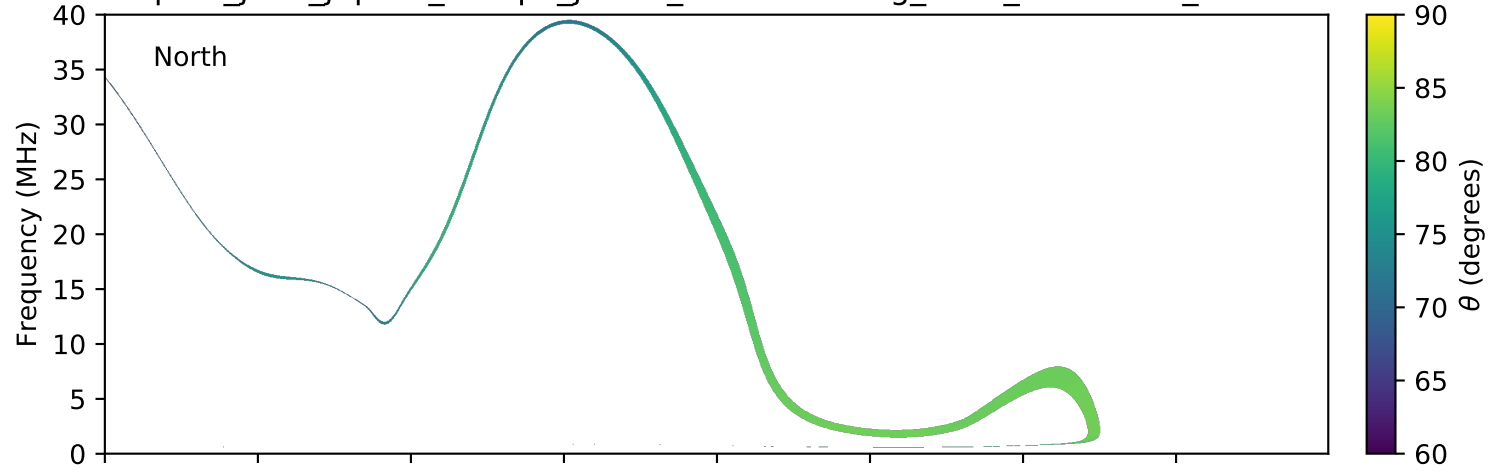
expres_juno_jupiter_europa_jrm09_lossc-wid1deg_3kev_20180126_v01.cdf
