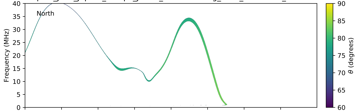
expres_juno_jupiter_europa_jrm09_lossc-wid1deg_3kev_20180125_v01.cdf
