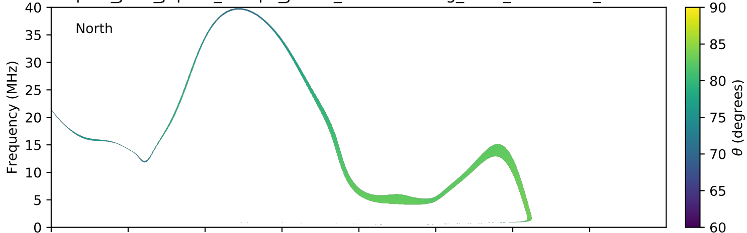
expres_juno_jupiter_europa_jrm09_lossc-wid1deg_3kev_20180124_v01.cdf
