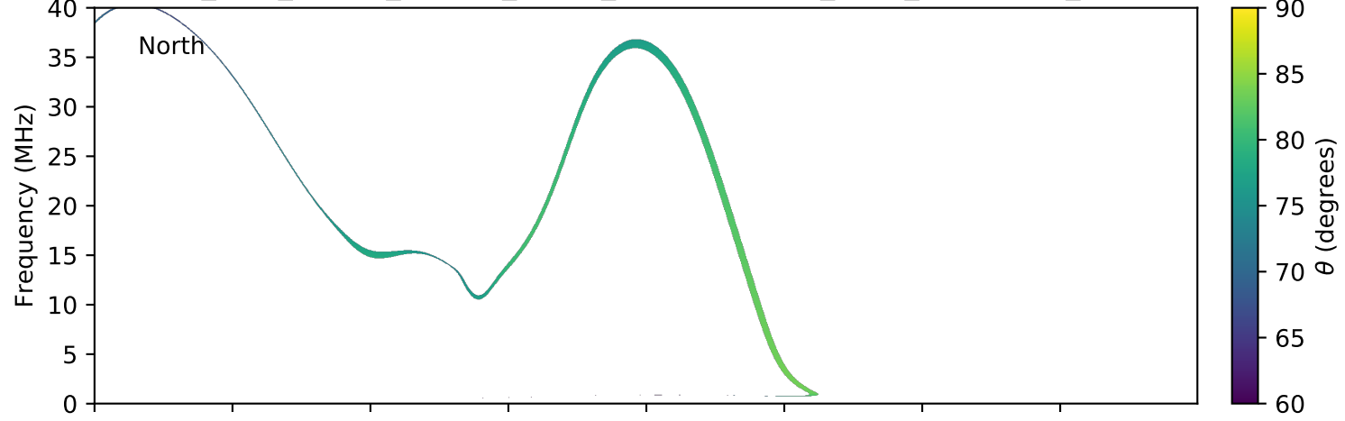
expres_juno_jupiter_europa_jrm09_lossc-wid1deg_3kev_20180123_v01.cdf
