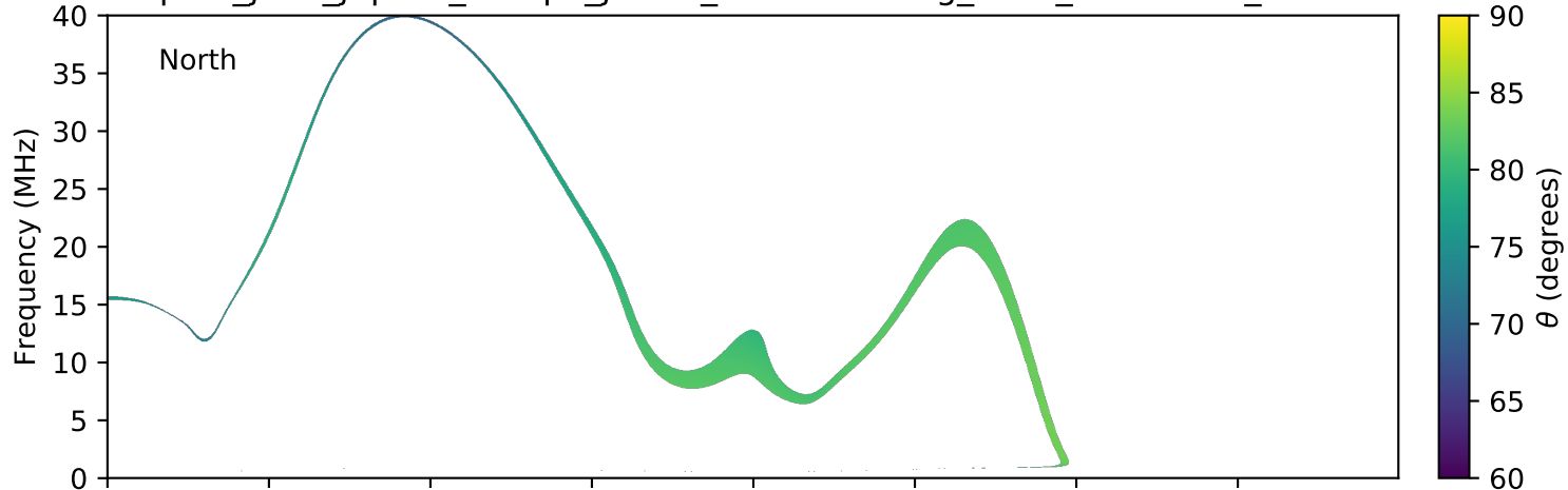
expres_juno_jupiter_europa_jrm09_lossc-wid1deg_3kev_20180122_v01.cdf
