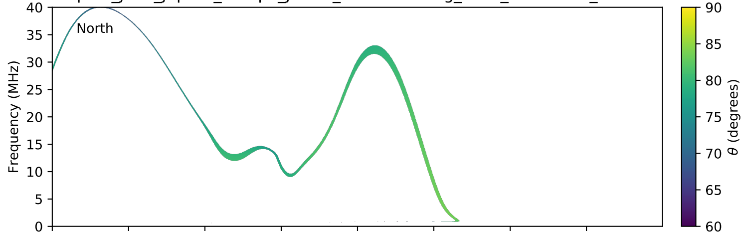
expres_juno_jupiter_europa_jrm09_lossc-wid1deg_3kev_20180118_v01.cdf
