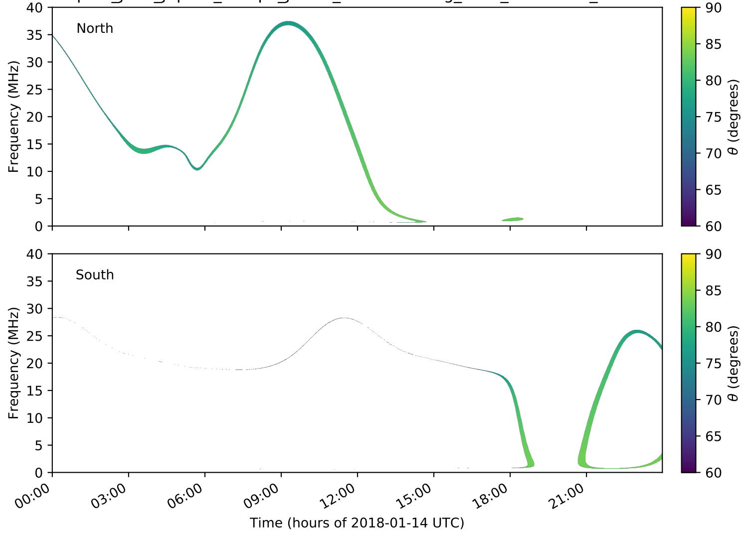
expres_juno_jupiter_europa_jrm09_lossc-wid1deg_3kev_20180114_v01.cdf
