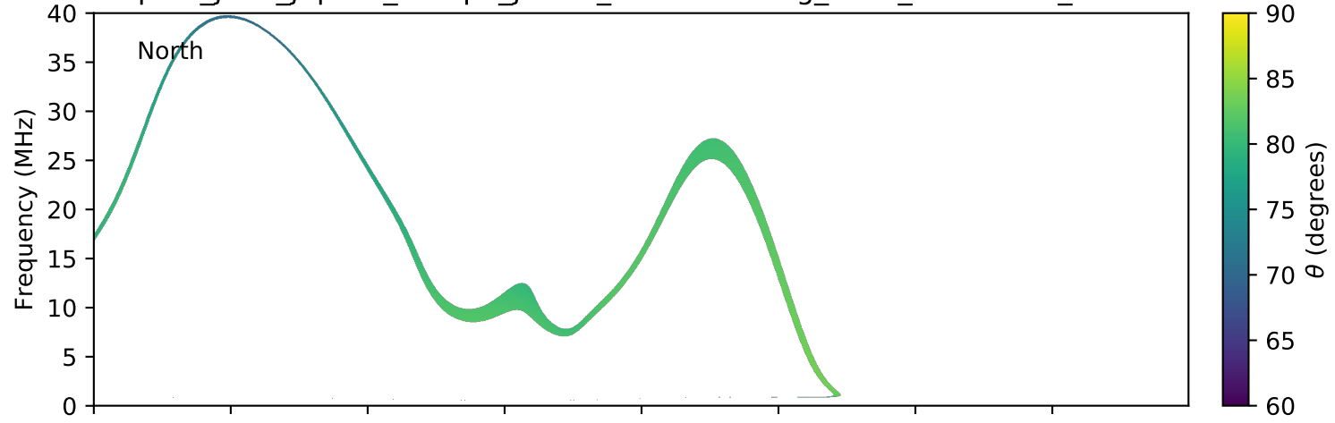
expres_juno_jupiter_europa_jrm09_lossc-wid1deg_3kev_20180113_v01.cdf
