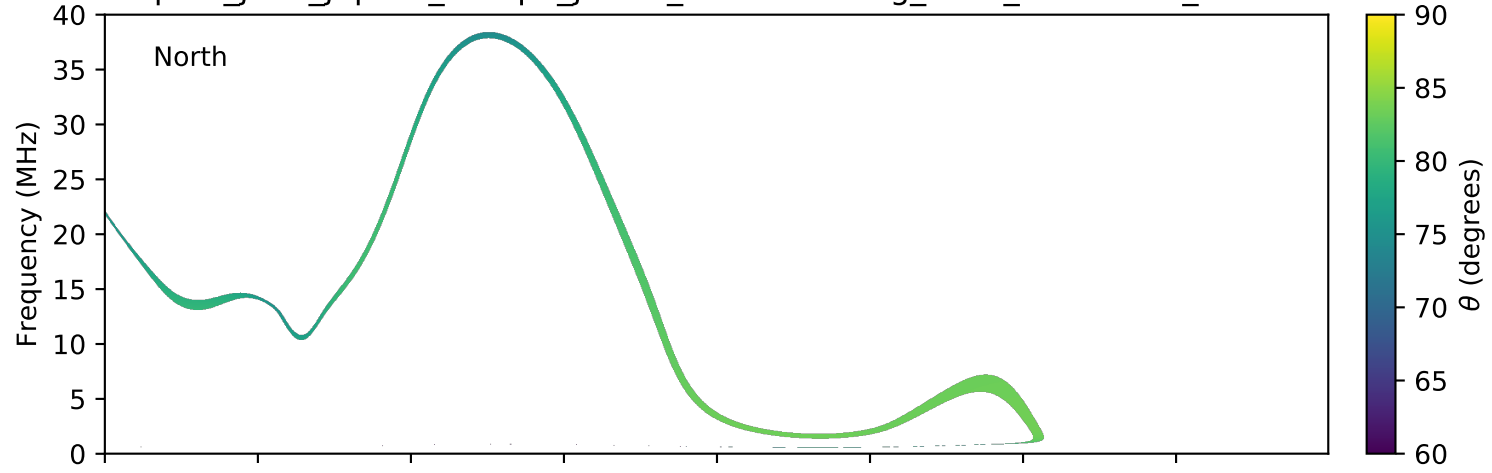
expres_juno_jupiter_europa_jrm09_lossc-wid1deg_3kev_20180112_v01.cdf
