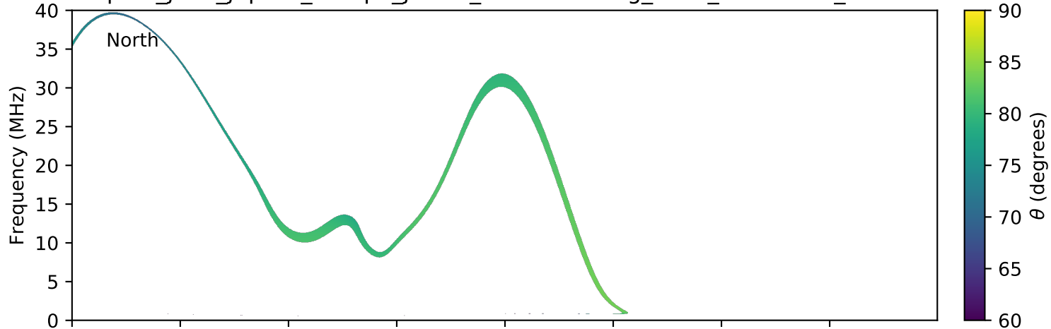
expres_juno_jupiter_europa_jrm09_lossc-wid1deg_3kev_20180111_v01.cdf
