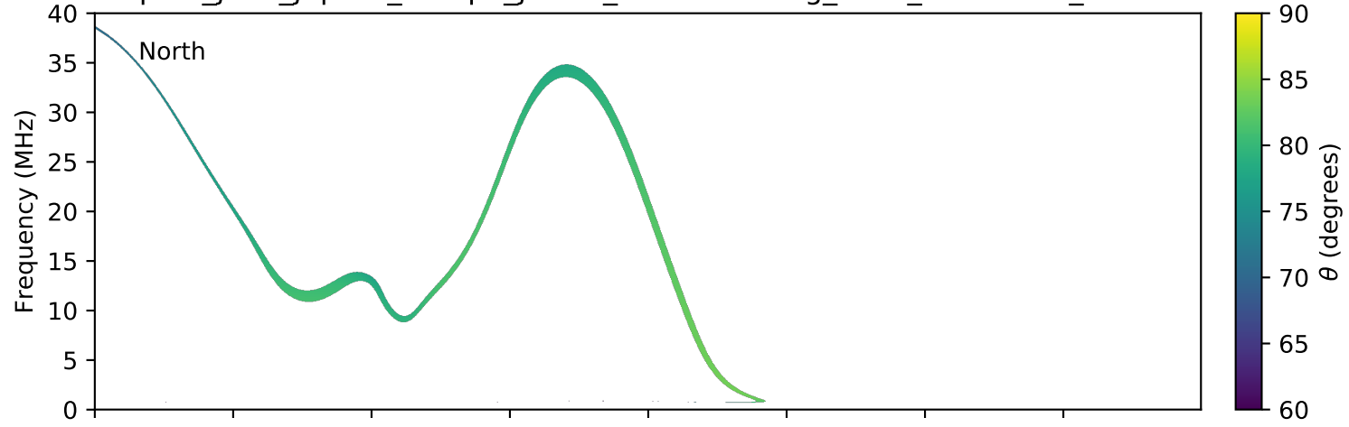
expres_juno_jupiter_europa_jrm09_lossc-wid1deg_3kev_20180109_v01.cdf
