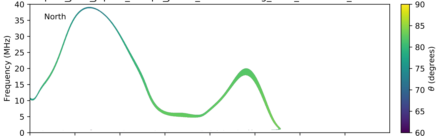
expres_juno_jupiter_europa_jrm09_lossc-wid1deg_3kev_20180108_v01.cdf
