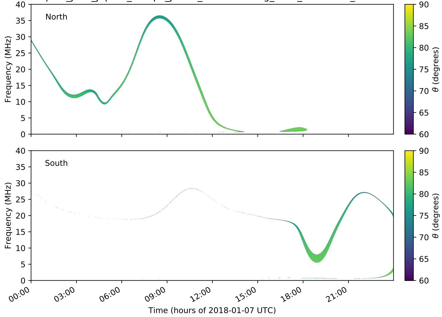
expres_juno_jupiter_europa_jrm09_lossc-wid1deg_3kev_20180107_v01.cdf
