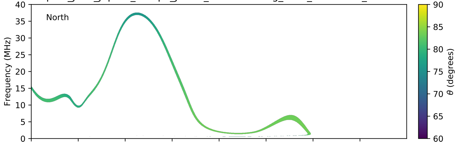
expres_juno_jupiter_europa_jrm09_lossc-wid1deg_3kev_20180105_v01.cdf
