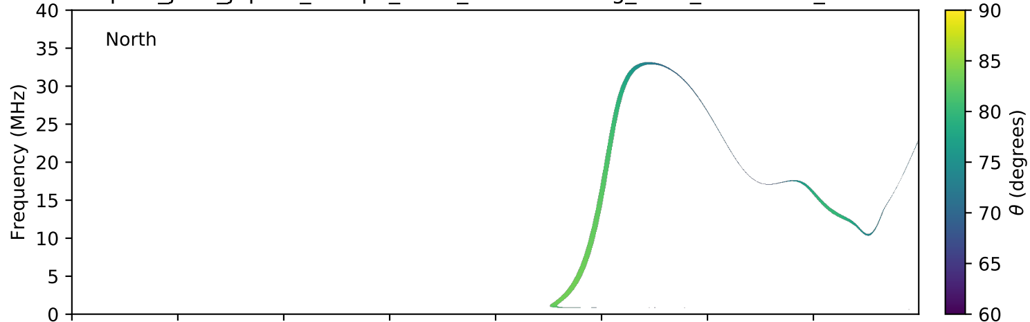
expres_juno_jupiter_europa_isaac_lossc-wid1deg_3kev_20180131_v01.cdf
