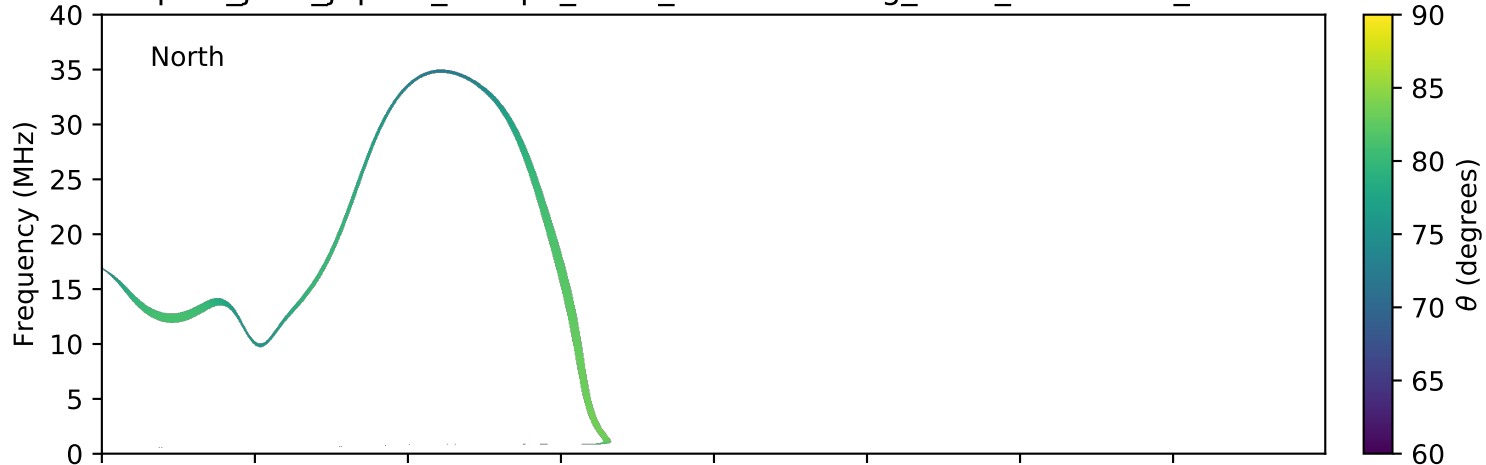
expres_juno_jupiter_europa_isaac_lossc-wid1deg_3kev_20180129_v01.cdf
