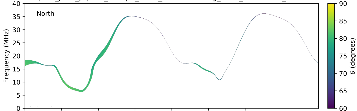
expres_juno_jupiter_europa_isaac_lossc-wid1deg_3kev_20180128_v01.cdf
