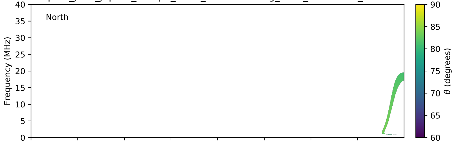
expres_juno_jupiter_europa_isaac_lossc-wid1deg_3kev_20180127_v01.cdf
