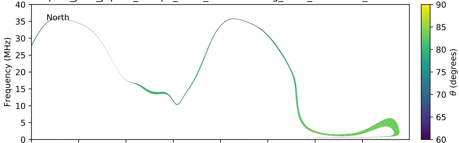
expres_juno_jupiter_europa_isaac_lossc-wid1deg_3kev_20180125_v01.cdf
