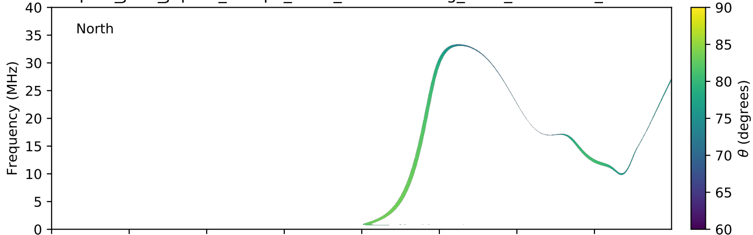
expres_juno_jupiter_europa_isaac_lossc-wid1deg_3kev_20180124_v01.cdf
