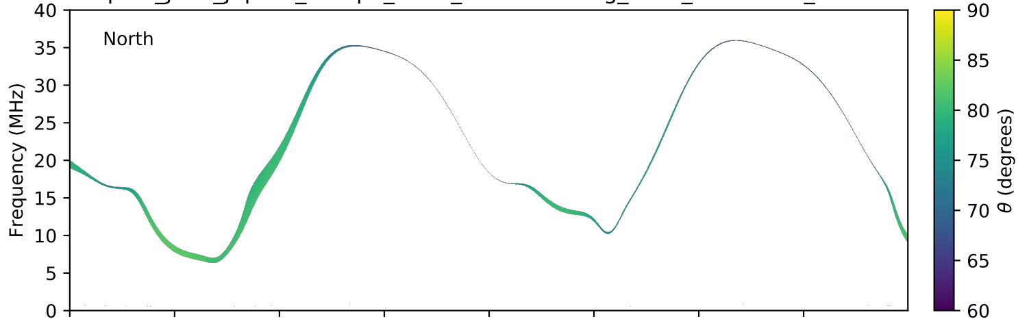
expres_juno_jupiter_europa_isaac_lossc-wid1deg_3kev_20180121_v01.cdf
