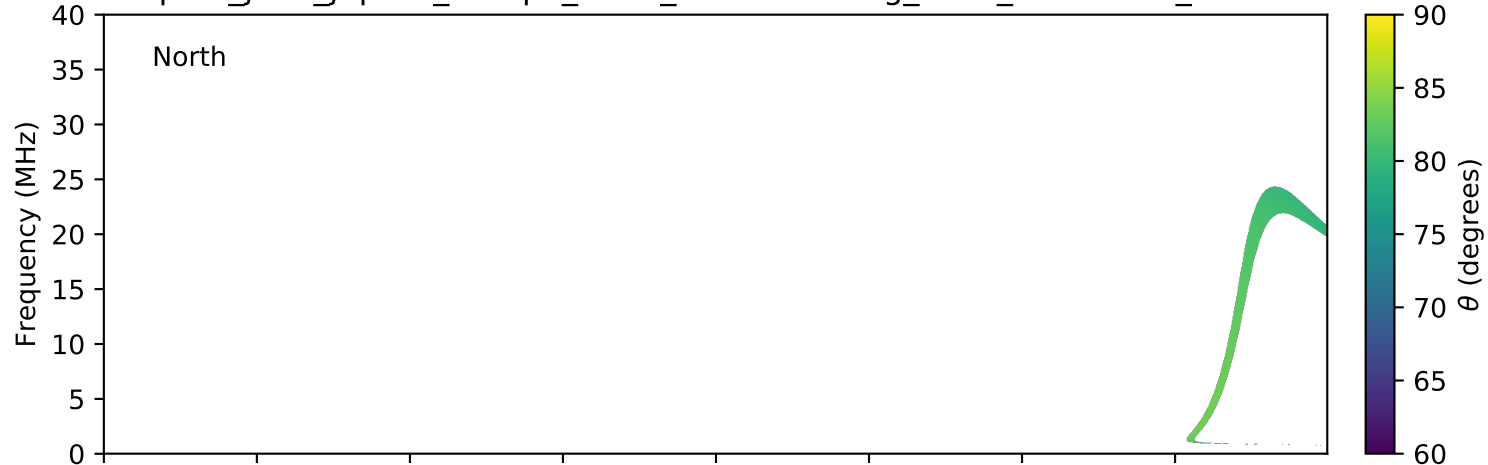
expres_juno_jupiter_europa_isaac_lossc-wid1deg_3kev_20180120_v01.cdf
