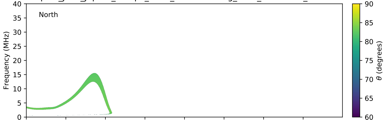
expres_juno_jupiter_europa_isaac_lossc-wid1deg_3kev_20180115_v01.cdf
