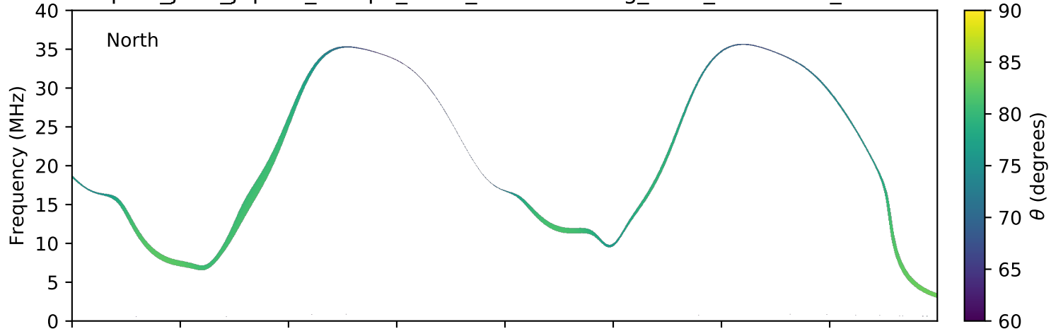
expres_juno_jupiter_europa_isaac_lossc-wid1deg_3kev_20180114_v01.cdf
