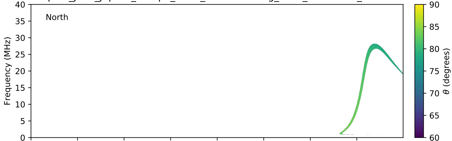
expres_juno_jupiter_europa_isaac_lossc-wid1deg_3kev_20180113_v01.cdf
