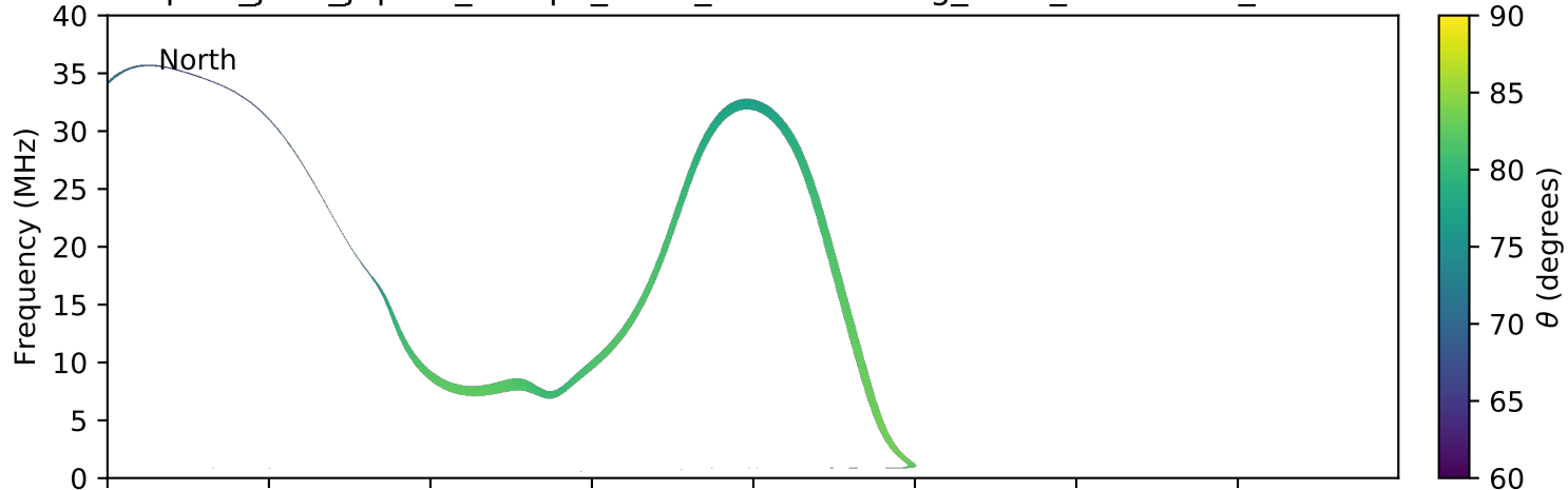
expres_juno_jupiter_europa_isaac_lossc-wid1deg_3kev_20180111_v01.cdf
