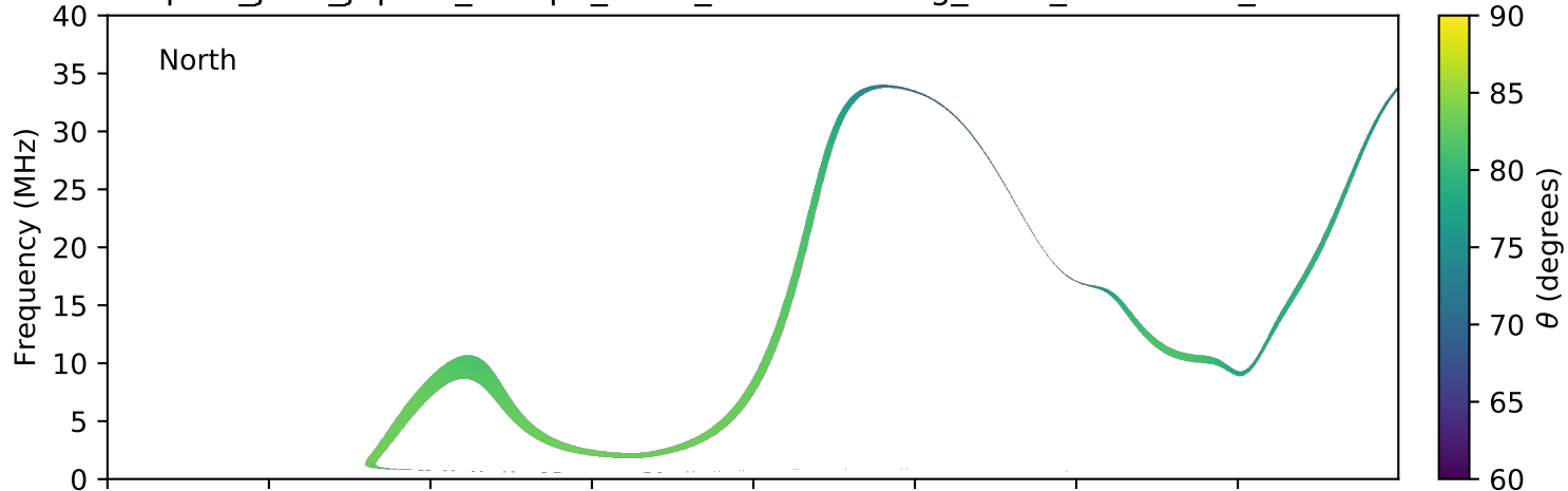
expres_juno_jupiter_europa_isaac_lossc-wid1deg_3kev_20180110_v01.cdf
