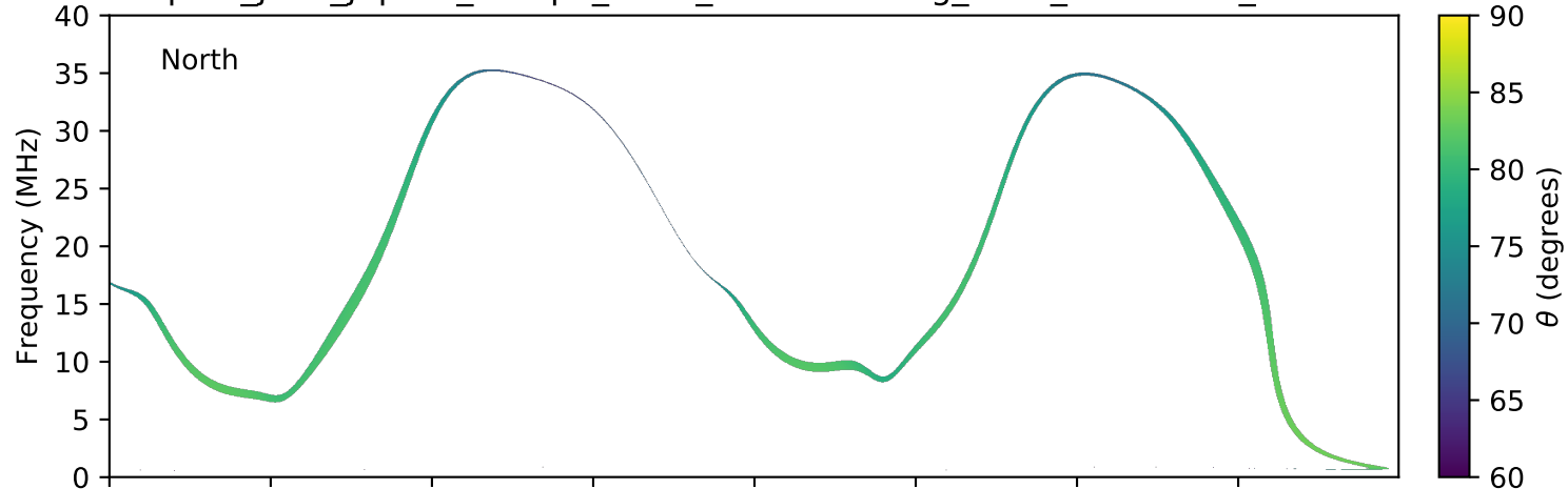
expres_juno_jupiter_europa_isaac_lossc-wid1deg_3kev_20180107_v01.cdf
