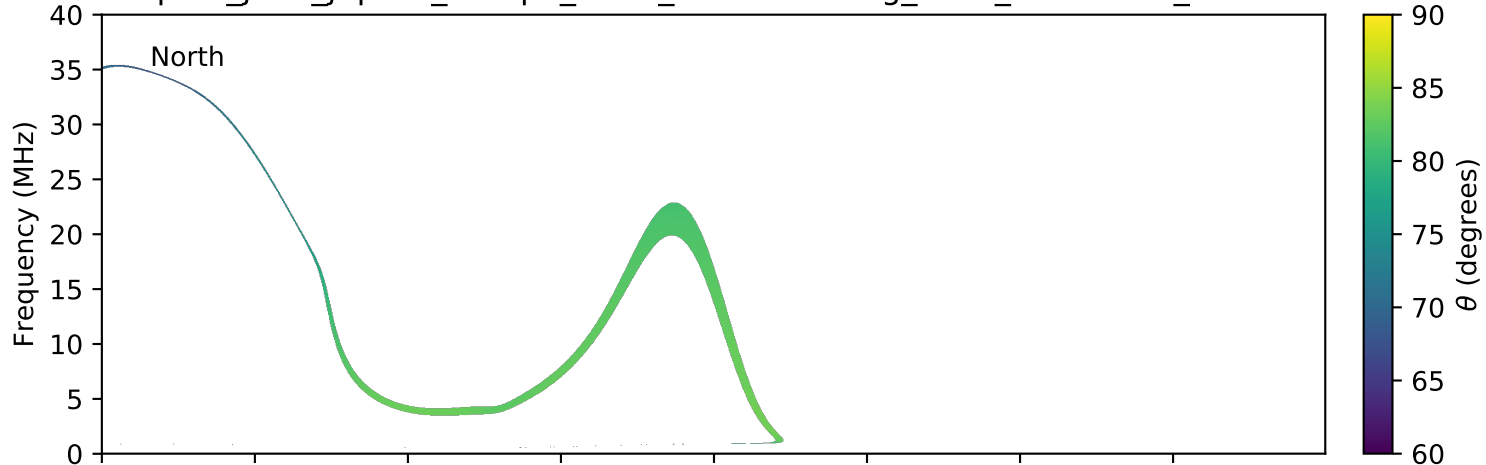
expres_juno_jupiter_europa_isaac_lossc-wid1deg_3kev_20180104_v01.cdf
